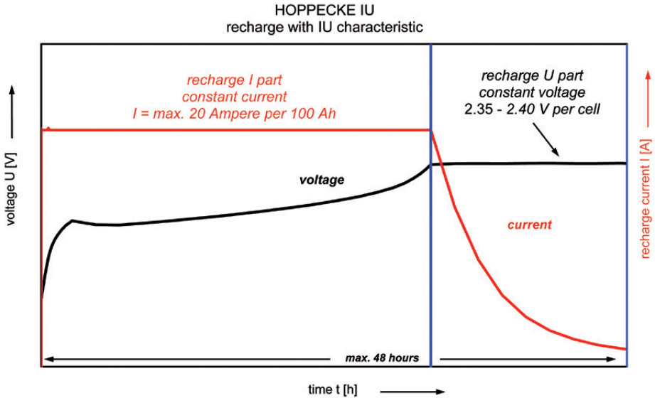
Fig. 9-1: IU characteristic
